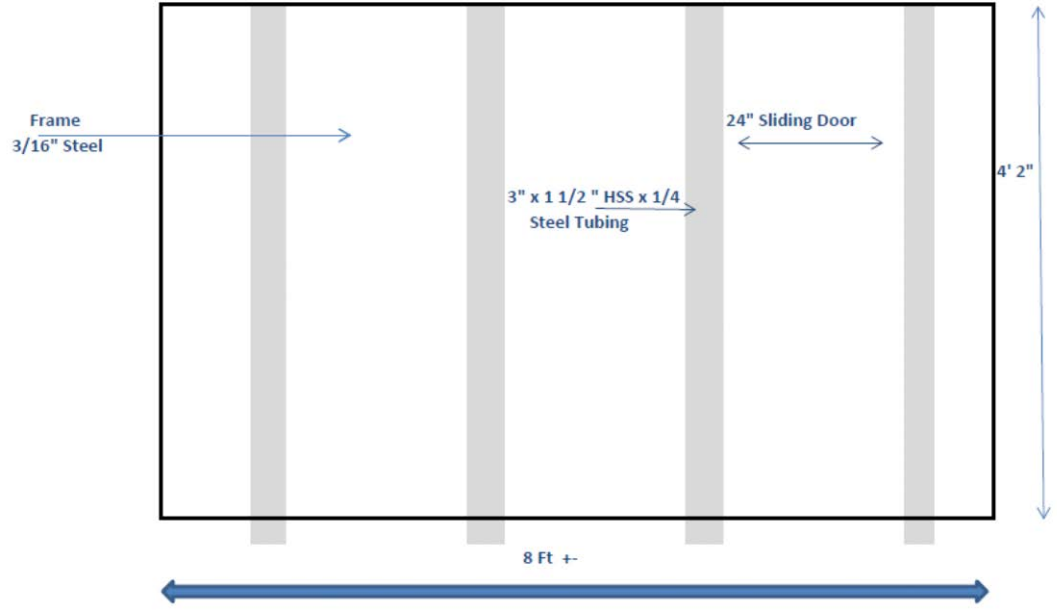
Details A - Rear Panel
