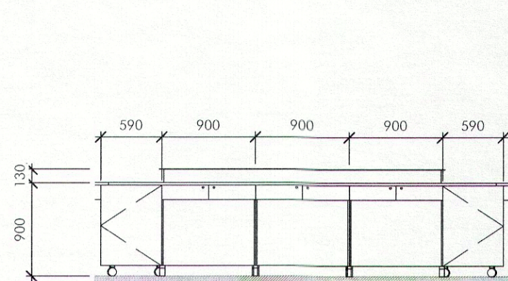
4 COUNCIL FRONT 2 A2.02 1:50
