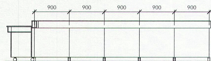
5 COUNCIL BACK 1 A2.02 1:50
