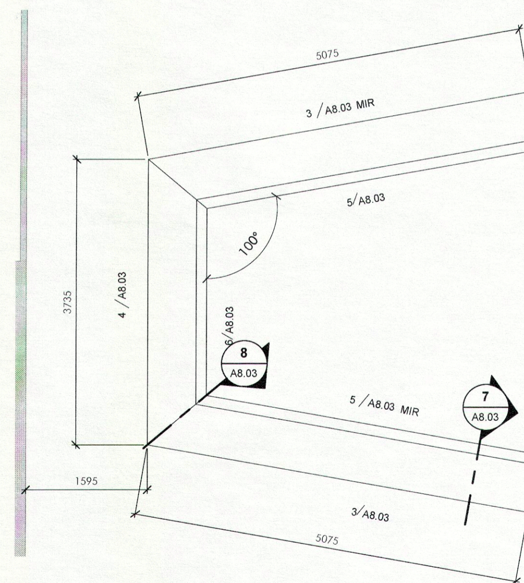
2 COUNCIL DESK - FLOOR PLAN A3.01 1:50
