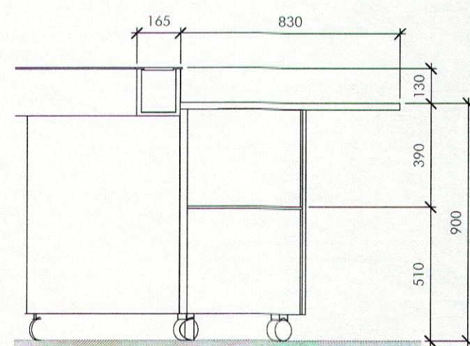
8 COUNCIL DESK SECTION 2 A8.03 1:20
