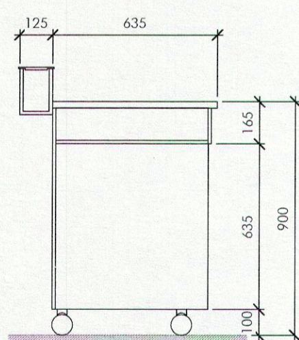
7 COUNCIL DESK SECTION 1 A8.03 1:20
