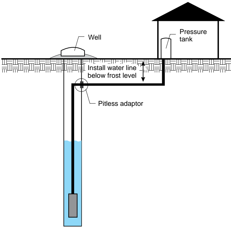
Figure 4-2, Pitless Adaptor
